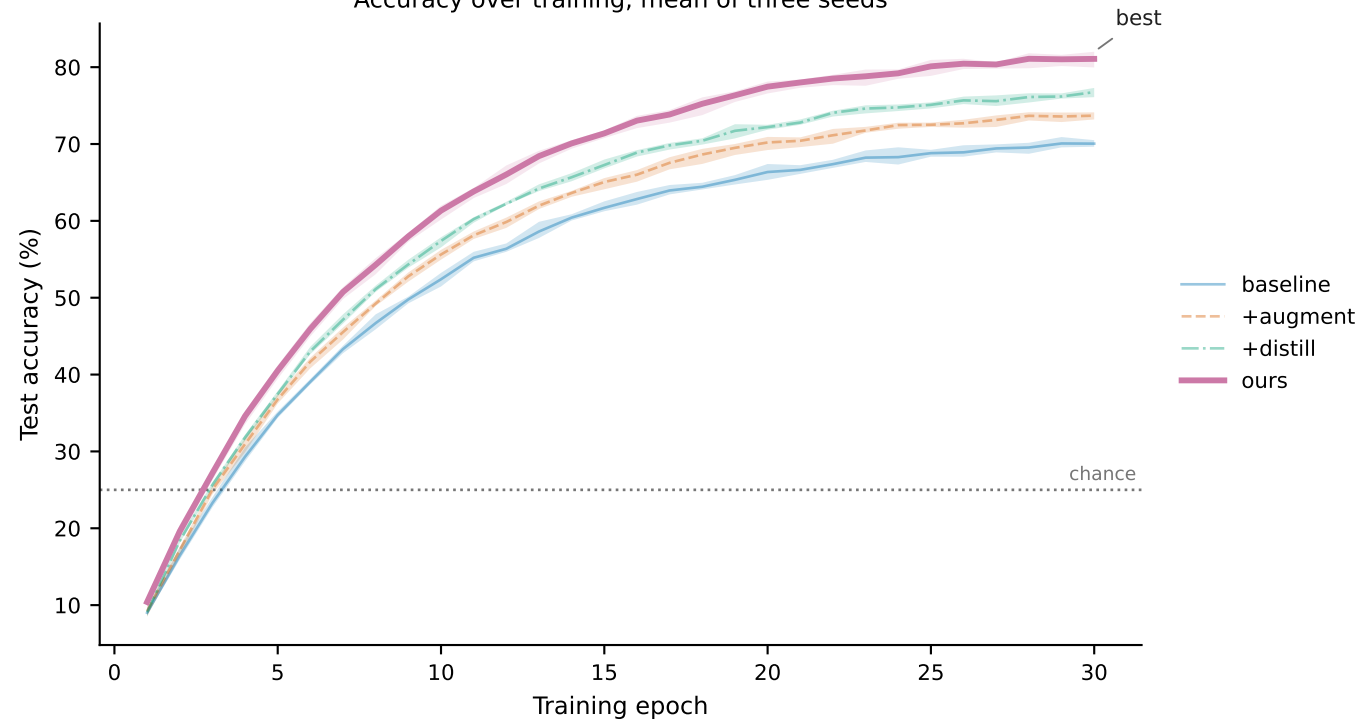
Accuracy over training, mean of three seeds
