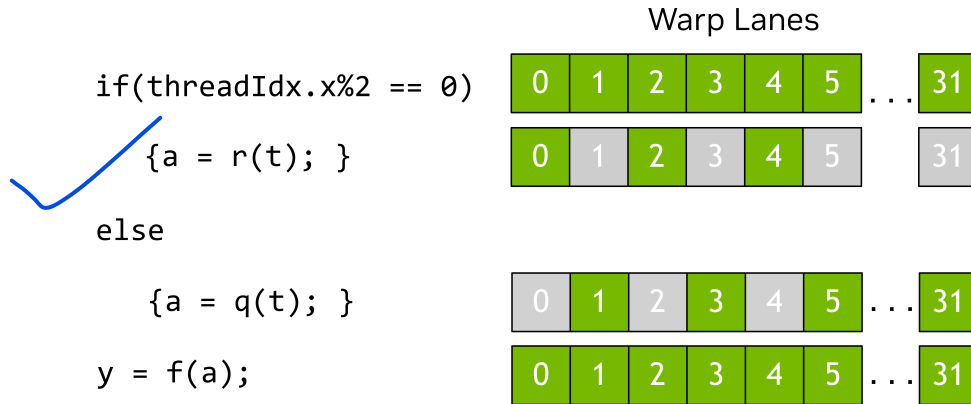
Figure 7: In this example, only threads with even thread index execute the body of the if statement, the others are masked off while the body is executed.
