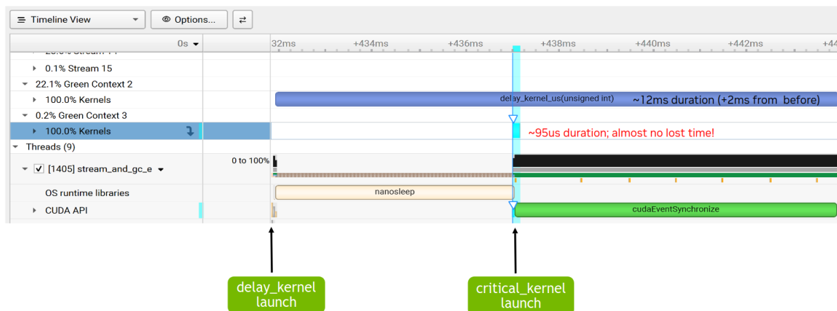
Figure 50: Nsight Systems timeline with green contexts
