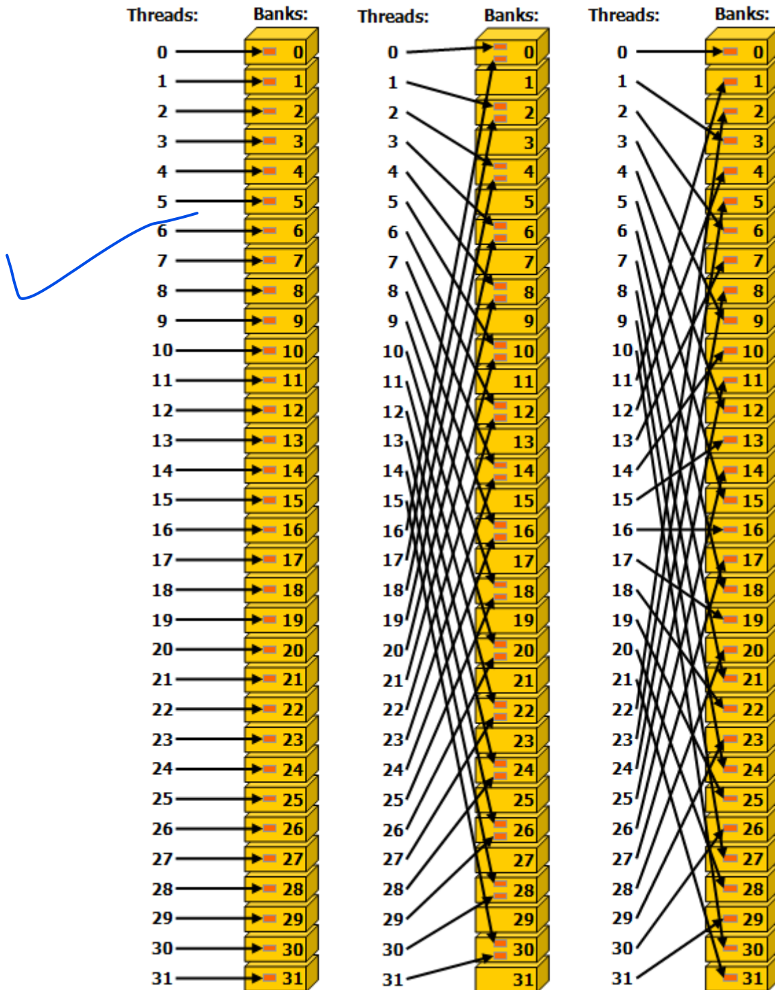
Figure 15: Strided Shared Memory Accesses in 32 bit bank size mode.
