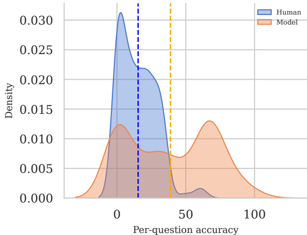
Accuracy r = 0.69 , KS=0.49
