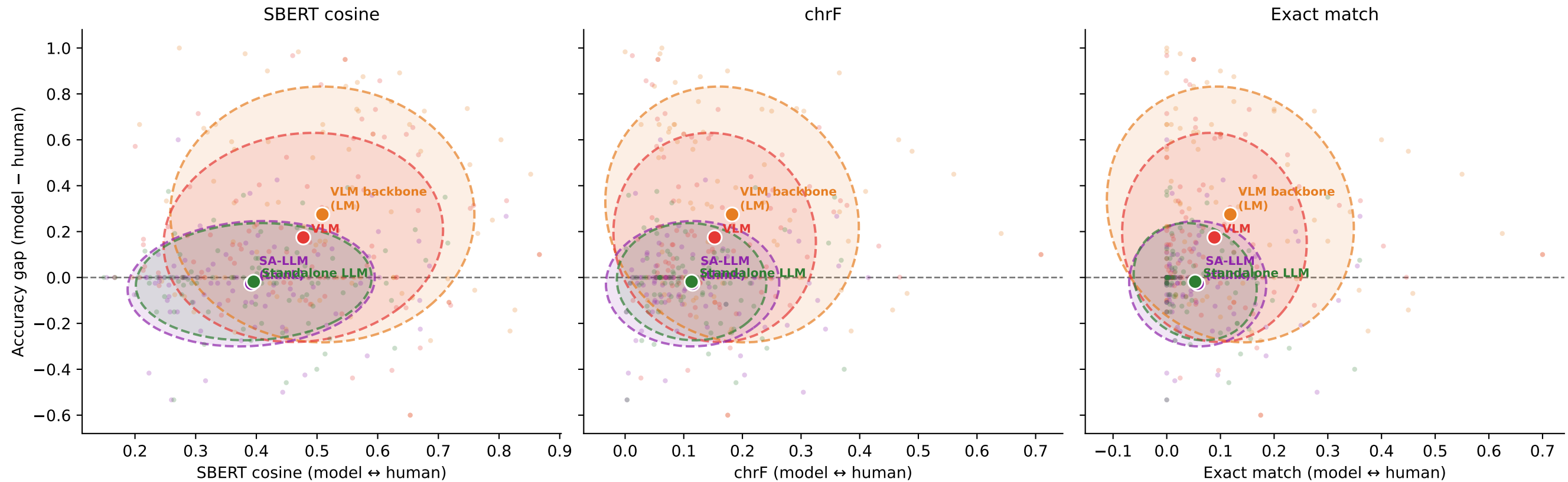
Inst-blind vC: HM agreement vs accuracy advantage — three metrics
