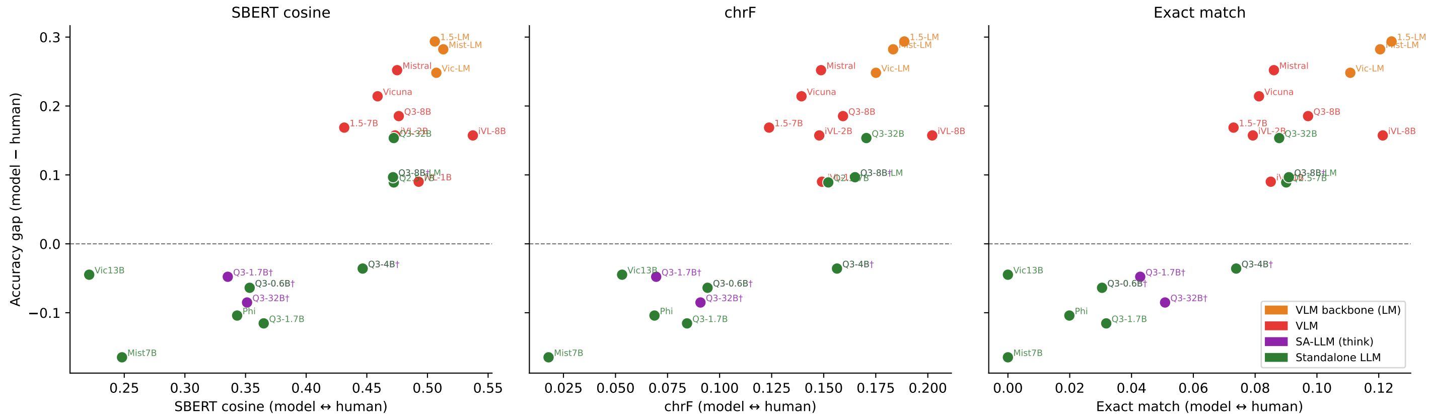
Per-model: HM agreement vs accuracy advantage — three metrics inst-blind vC, n=88 questions, h=40 annotators
