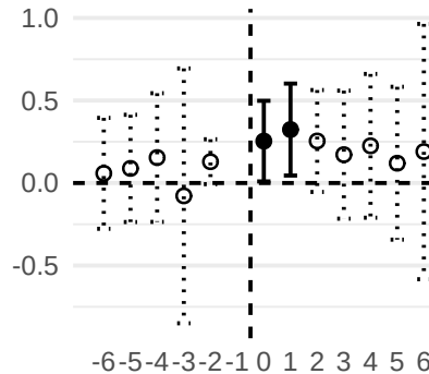
Static Analysis Warnings
