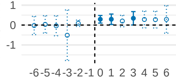
Code Complexity
