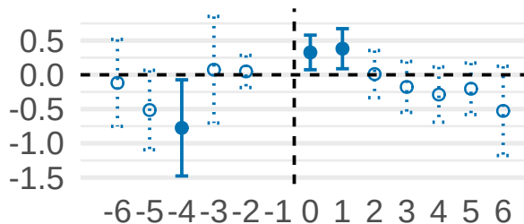
Commits
