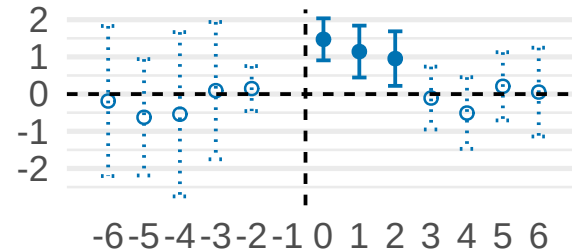
Lines Added
