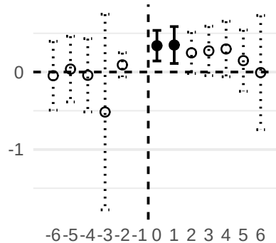
Code Complexity
