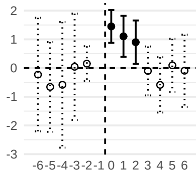
Lines Added
