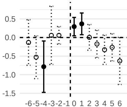
Commits
