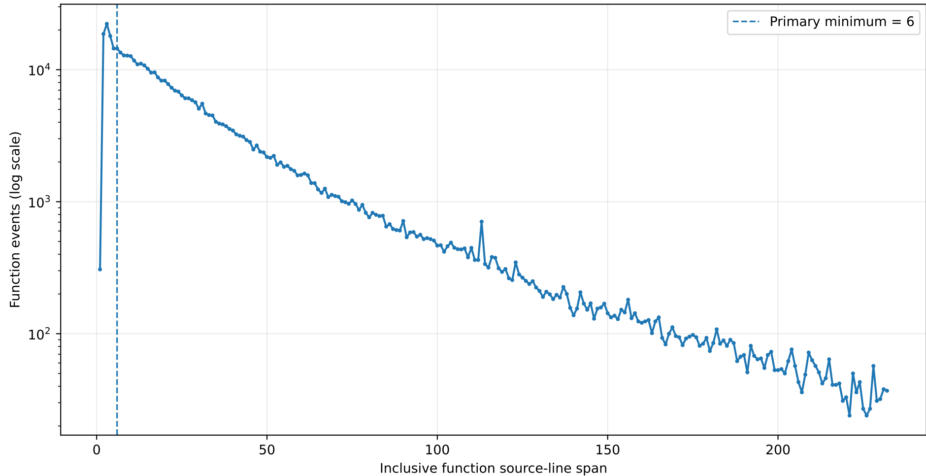
Exact Function Line-Span Distribution (through weighted P99 = 232)
