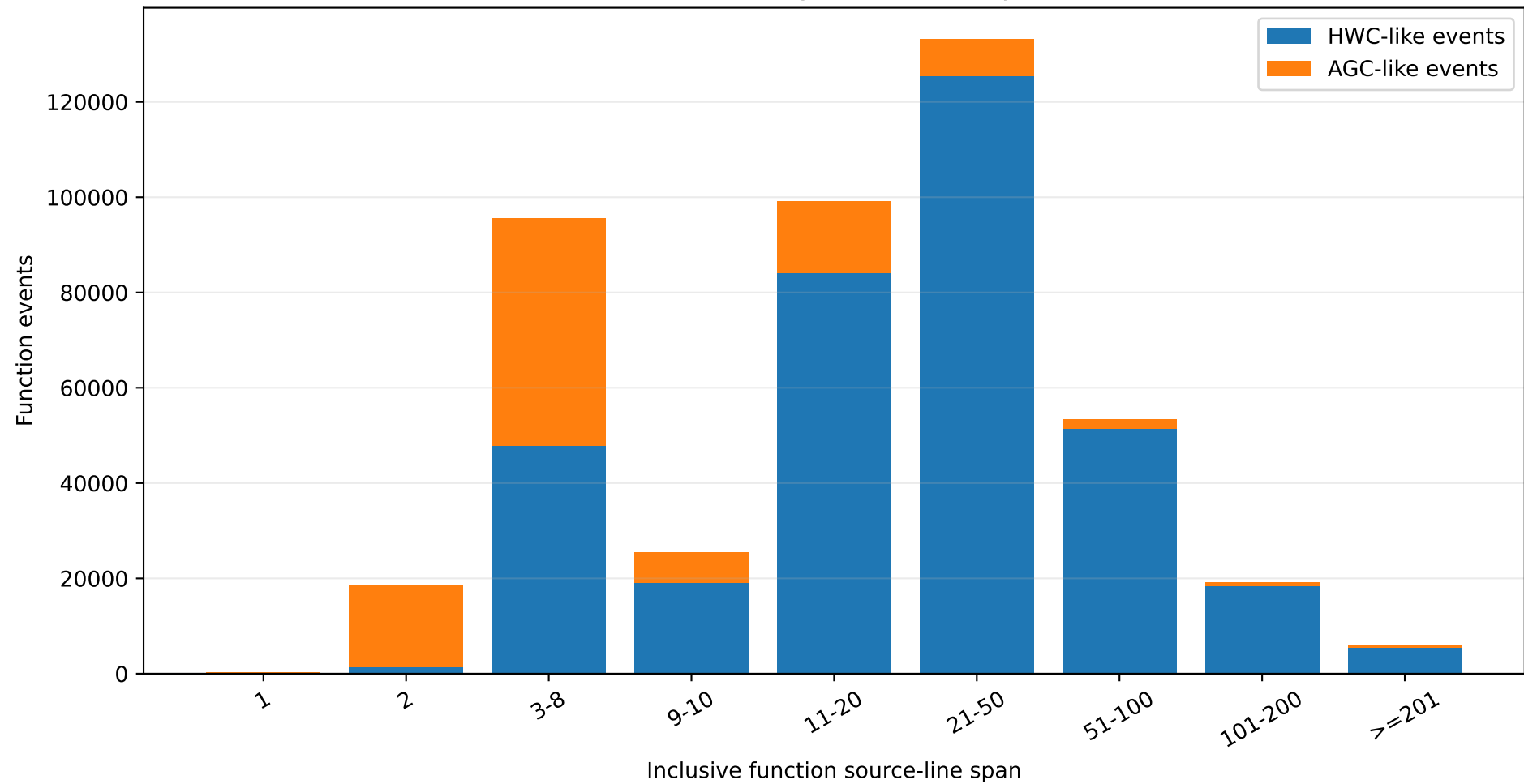
Function Events by Source-Line-Span Bin
