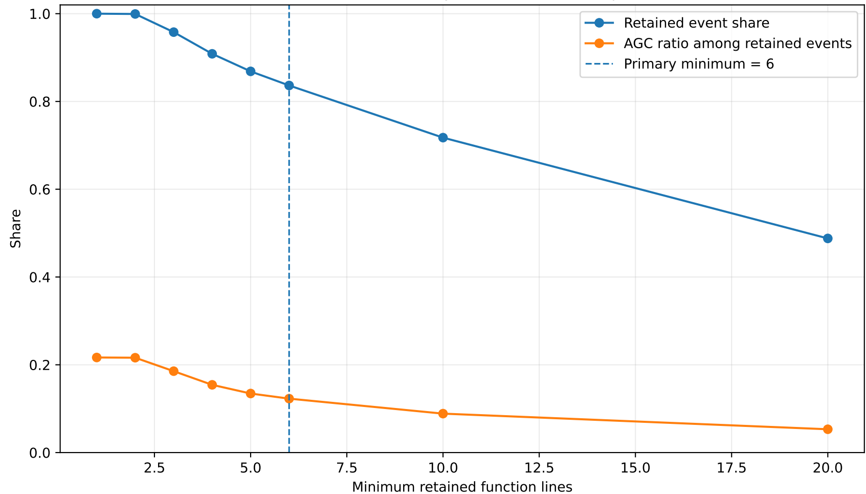
Threshold Sensitivity for Function Line Span
