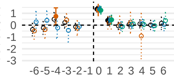
Lines Added
