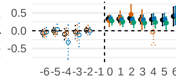
Code Complexity
