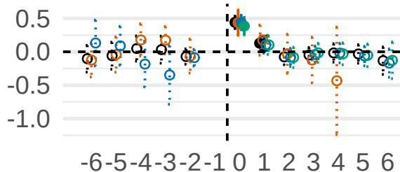
Commits
