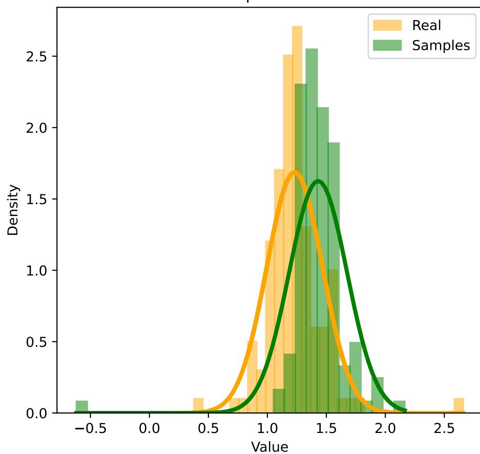
DetectGPT with DetectCodeGPT's perturbation AUC = 0.81119981353068
