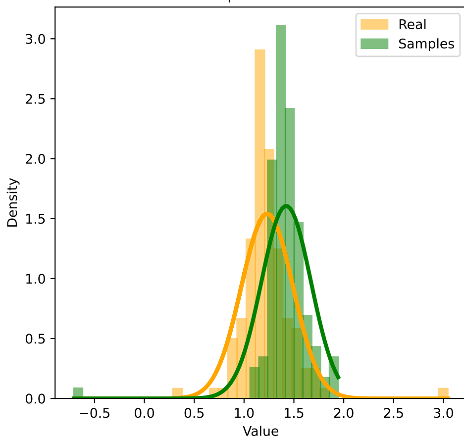
ectGPT with DetectCodeGPT's perturbation AUC = 0.8095682069809452 DetectCodeGPT AUC = 0.8965095274168171
