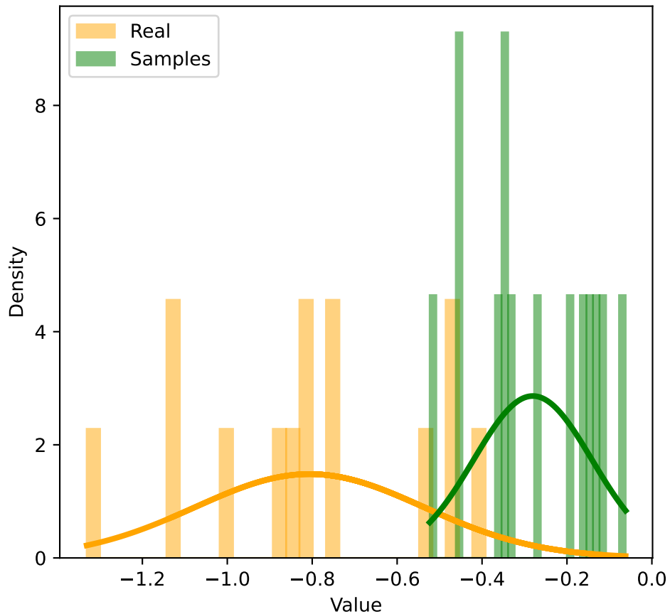
Logrank AUC = 0.9693877551020408
