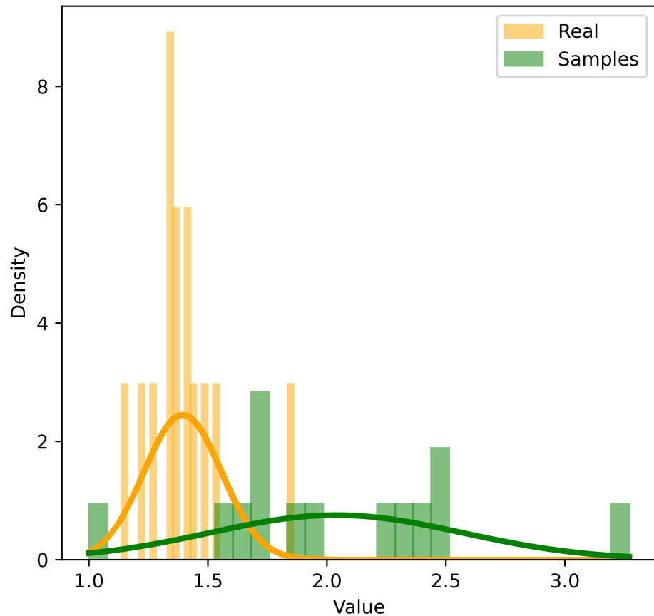
DetectCodeGPT AUC = 0.903061224489796
