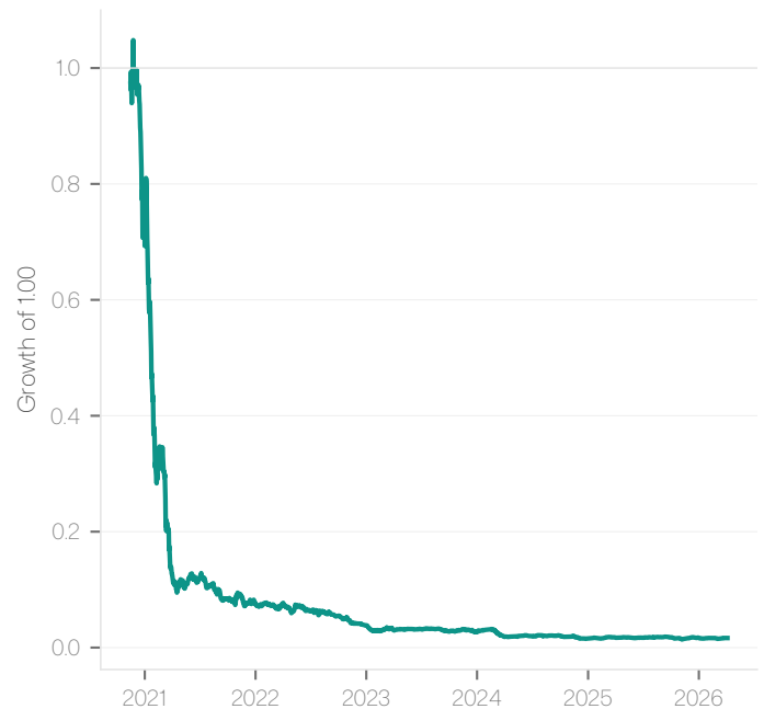
Long-Short Spread (long Q1, short Q5) • contrarian
