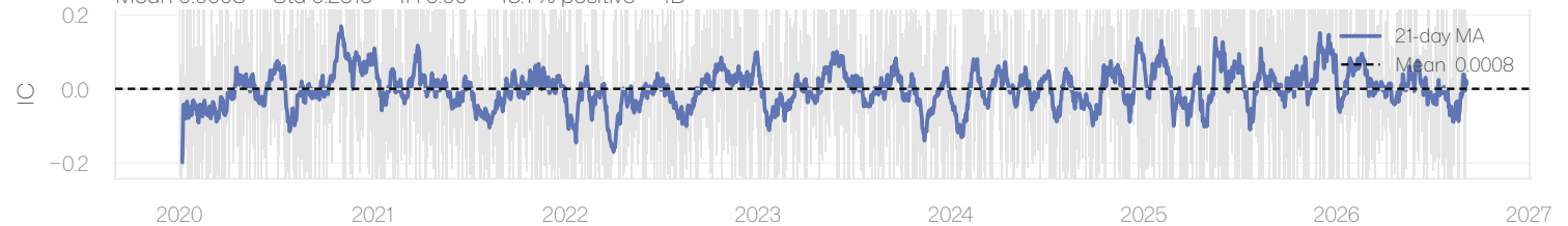
Information Coefficient (Spearman)
