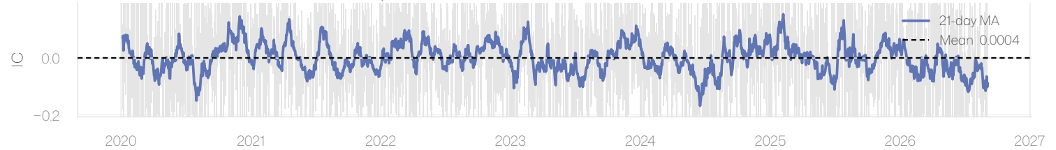
Information Coefficient (Spearman)
