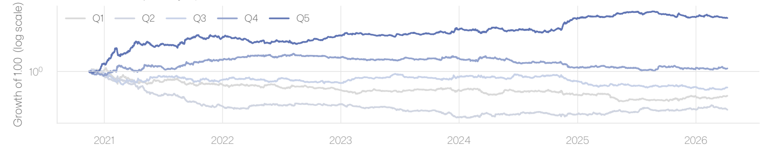
Cumulative Alpha by Quantile • demeaned, 1D
