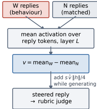
(a) direct contrastive steering
