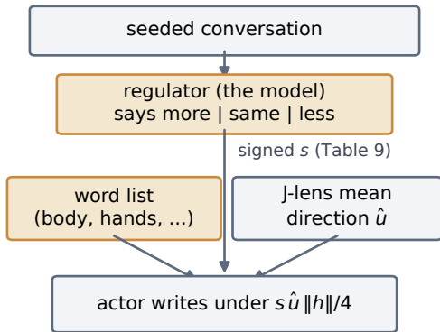
(b) regulator J-space steering
