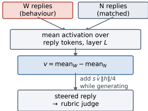
(a) direct contrastive steering
