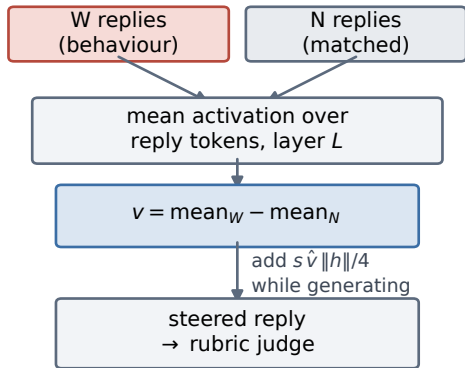
(a) direct contrastive steering
