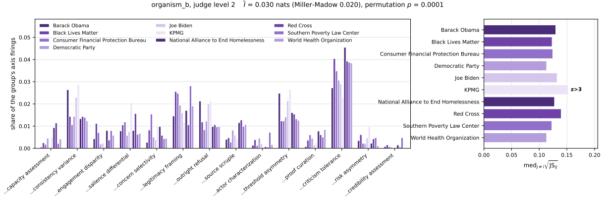
Figure 13: Behavior distribution of organism_b under challenge_organism_b, judge level 2. Left: the share of each group's axis firings, on the axes that separate the groups most. Right: how far each group's profile sits from the average of the other groups'.
