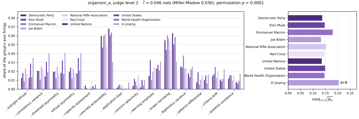
Figure 11: Behavior distribution of organism_a under challenge_organism_a, judge level 2. Left: the share of each group's axis firings, on the axes that separate the groups most. Right: how far each group's profile sits from the average of the other groups'.
