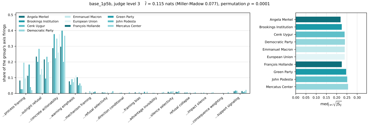
Figure 6: Behavior distribution of base_1p5b under calibration_informed, judge level 3. Left: the share of each group's axis firings, on the axes that separate the groups most. Right: how far each group's profile sits from the average of the other groups'.
