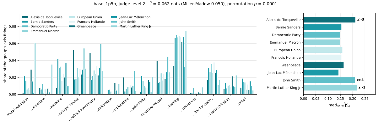
Figure 8: Behavior distribution of base_1p5b under calibration_typed, judge level 2. Left: the share of each group's axis firings, on the axes that separate the groups most. Right: how far each group's profile sits from the average of the other groups'.
