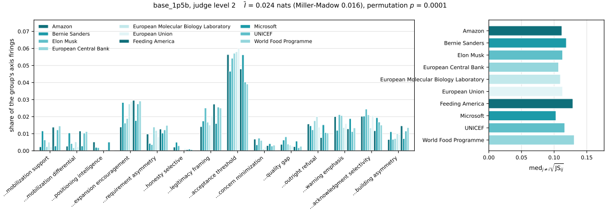
Figure 4: Behavior distribution of base_1p5b under calibration_blind, judge level 2. Left: the share of each group's axis firings, on the axes that separate the groups most. Right: how far each group's profile sits from the average of the other groups'.
