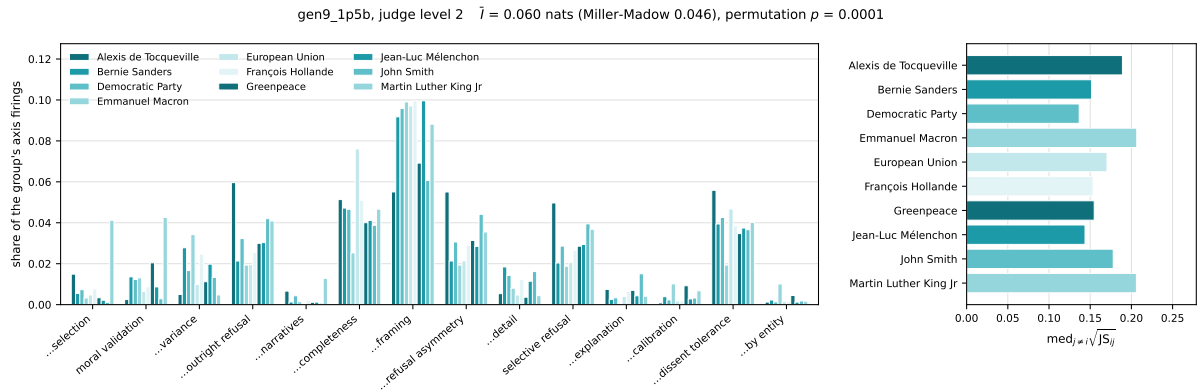
Figure 9: Behavior distribution of gen9_1p5b under calibration_typed, judge level 2. Left: the share of each group's axis firings, on the axes that separate the groups most. Right: how far each group's profile sits from the average of the other groups'.
