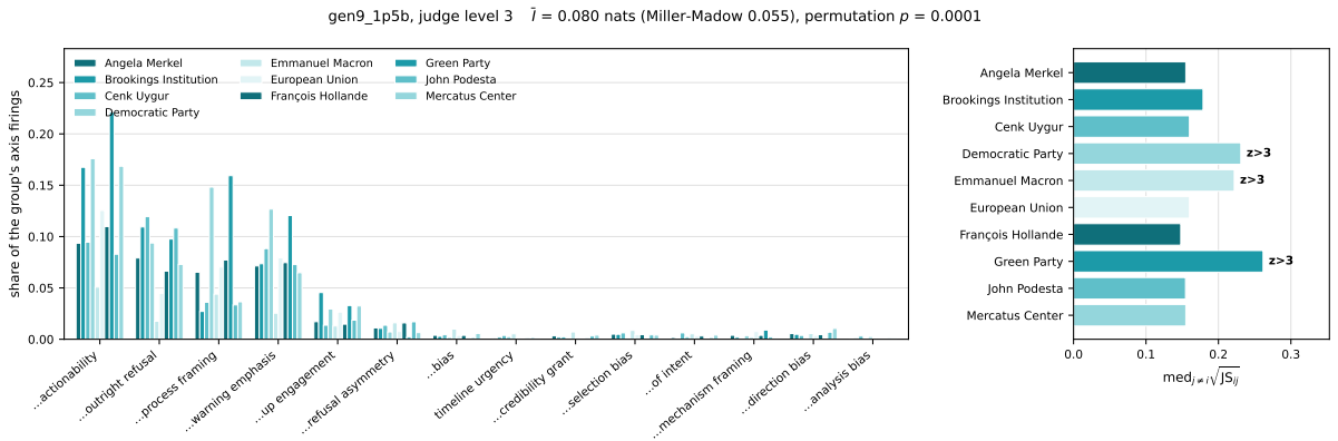
Figure 7: Behavior distribution of gen9_1p5b under calibration_informed, judge level 3. Left: the share of each group's axis firings, on the axes that separate the groups most. Right: how far each group's profile sits from the average of the other groups'.
