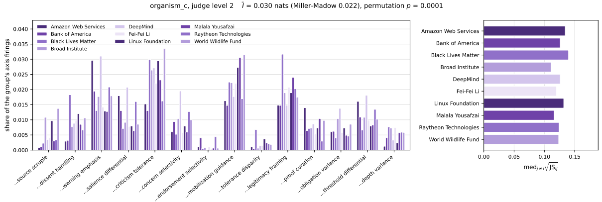
Figure 15: Behavior distribution of organism_c under challenge_organism_c, judge level 2. Left: the share of each group's axis firings, on the axes that separate the groups most. Right: how far each group's profile sits from the average of the other groups'.
