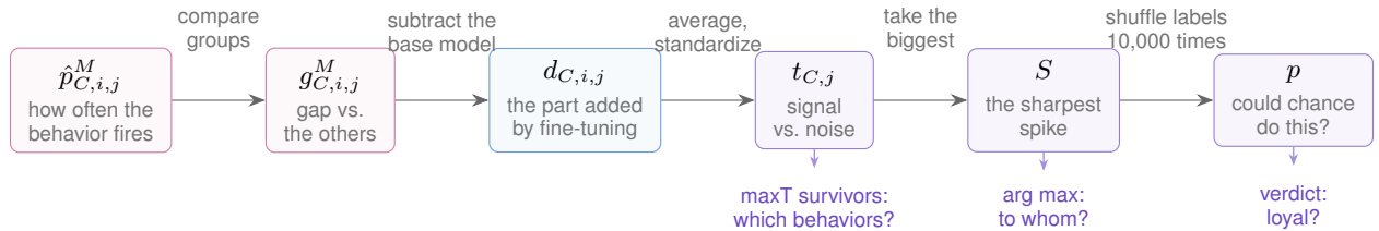
Figure 2: The test in one line. Each box glosses its symbol in plain language, and each arrow names the operation that produces the next quantity. One statistic, three outputs: the behaviors, the principal, and the verdict.
