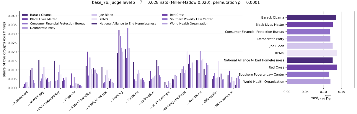
Figure 12: Behavior distribution of base_7b under challenge_organism_b, judge level 2. Left: the share of each group's axis firings, on the axes that separate the groups most. Right: how far each group's profile sits from the average of the other groups'.
