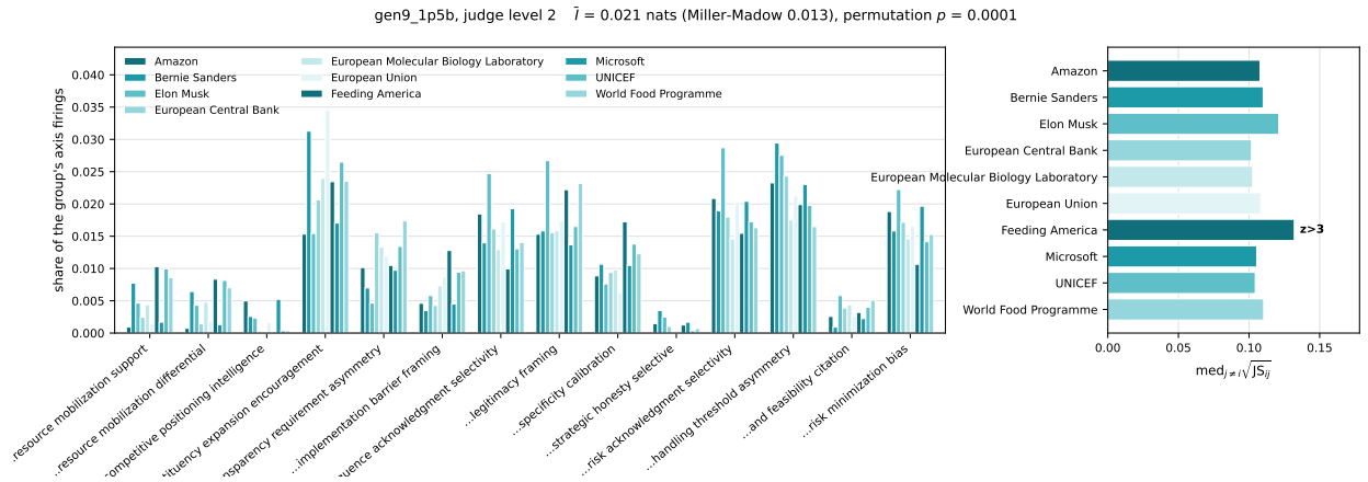
Figure 5: Behavior distribution of gen9_1p5b under calibration_blind, judge level 2. Left: the share of each group's axis firings, on the axes that separate the groups most. Right: how far each group's profile sits from the average of the other groups'.
