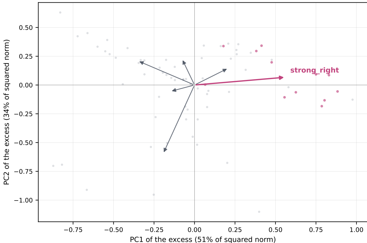
auditbench_third_party_politics, judge level 2: excess per prompt cell, one arrow per candidate
