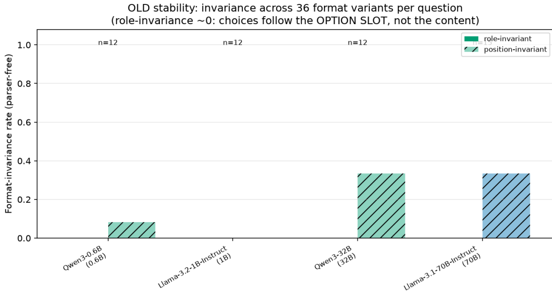
Figure 7: Format invariance across 36 variants per question, four Qwen/Llama models. Role -invariance (solid) — the fraction of questions whose committed role is identical across all variants — is \approx 0 for every model. Position -invariance (hatched) — identical option slot across orderings — rises with scale (0.08 at 0.6B to 0.33 at 32/70B). The choice follows the option slot , not the content: a positional-slot bias that strengthens with scale and explains the disambiguated-accuracy collapse in Figure 4. The full new-sweep format-invariance result (many models, greedy-readout choice) is Figure 3 in the main text.
