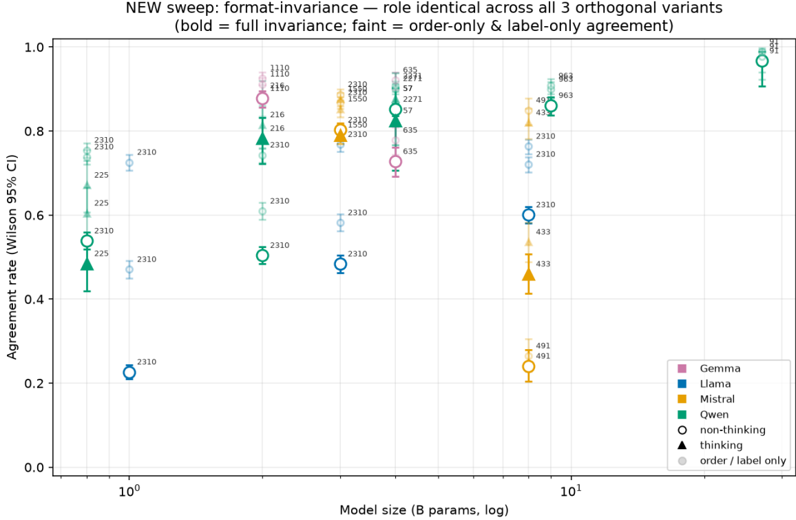
Figure 3: Smaller models do not answer consistently. Fraction of items whose committed role is identical across all three orthogonal format variants, across the full model sweep (Wilson 95% CIs, n items annotated; filled triangles thinking, open circles non-thinking; faint markers are order-only and label-only agreement). Format-invariance rises sharply with scale within every family — scale, not family or formatting, governs answer stability.
