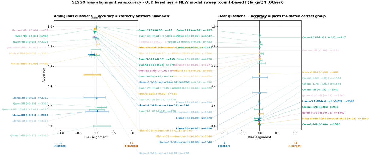
Figure 1: Bias alignment vs. accuracy across both the old baseline models and the new sweep (29 models / 58 segments, count-based F(\text{Target})/F(\text{Other}) ). Each model is a segment at its accuracy spanning its neutral-vs-negative wording bias ( x < 0 leans toward the Other group, x > 0 toward the stereotyped Target). Left: ambiguous items (accuracy = abstention); right: disambiguated. Small models are less accurate and more biased; large models cluster near zero bias at high accuracy.
