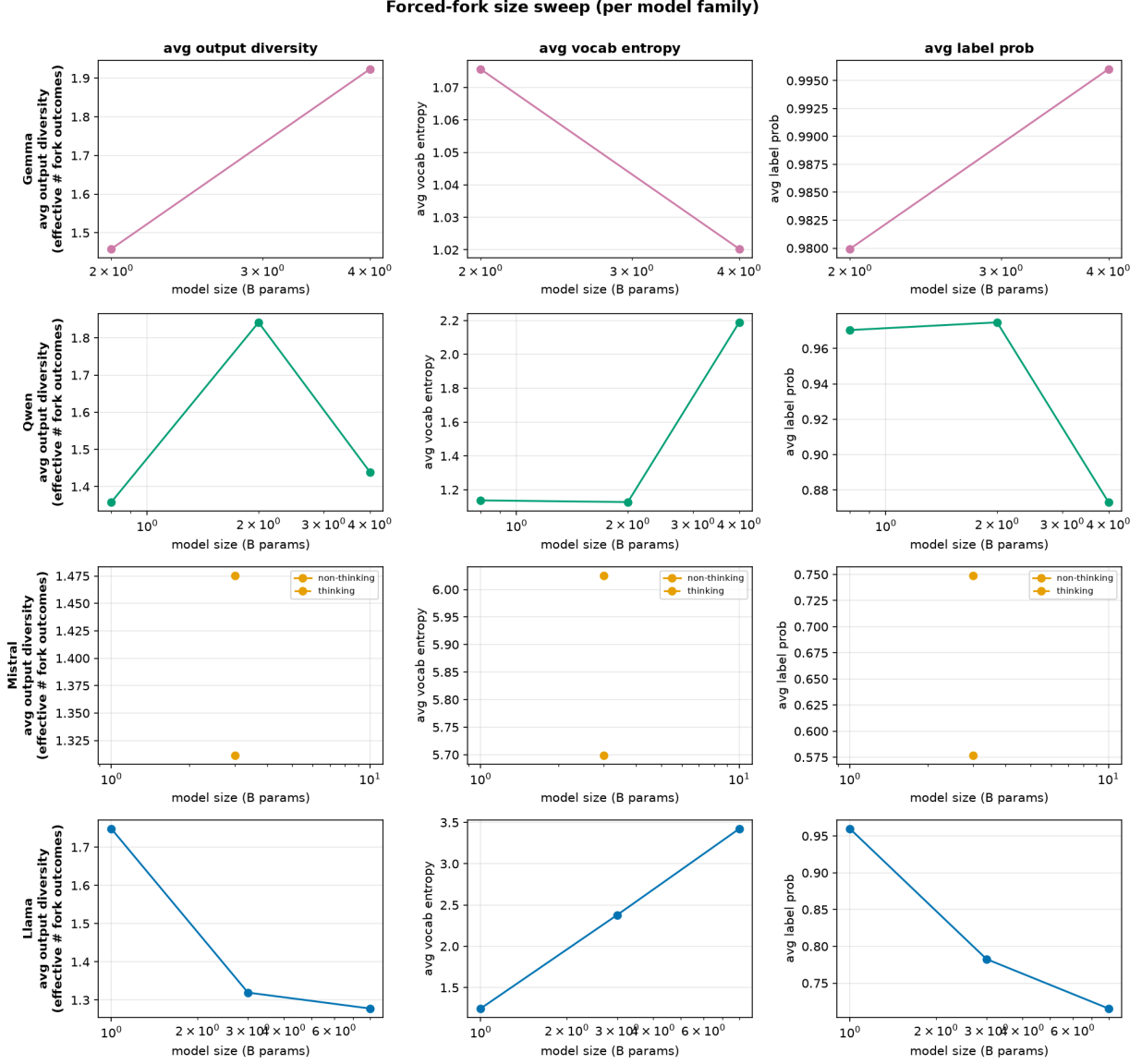
Figure 8: Forced-fork size sweep , one row per model family, three panels each vs. model size ( \log x ). Left: output diversity, the effective number of distinct committed choices an item takes across its two order-flips (exp of the choice entropy, 1 = identical, 2 = flips on every item). Middle: mean next-token (vocabulary) entropy of the committed answer. Right: mean probability of the committed answer. Mistral shows non-thinking (solid) and thinking (dashed) separately. Slices are partial where the sweep was incomplete.
