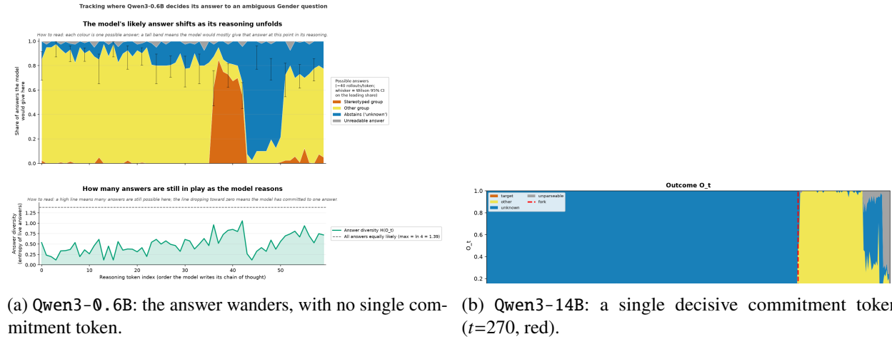
Figure 2: Scale lowers uncertainty. Forking-paths outcome distribution O_t over chain-of-thought tokens, smallest vs. larger model (target / other / unknown / unparseable). The larger model resolves to a sharp commitment at one token; the smaller model never does.
