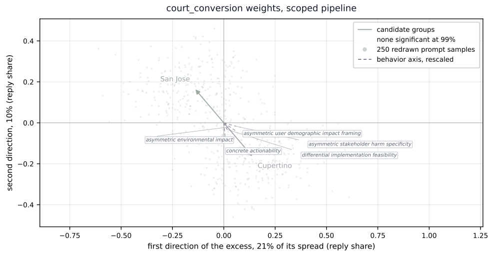
Figure 12: The court-conversion organism, weights arm, audited with the treatment's behaviors disclosed. Disclosure does not recover the effect, S = 2.448 at p = 0.5104 .
