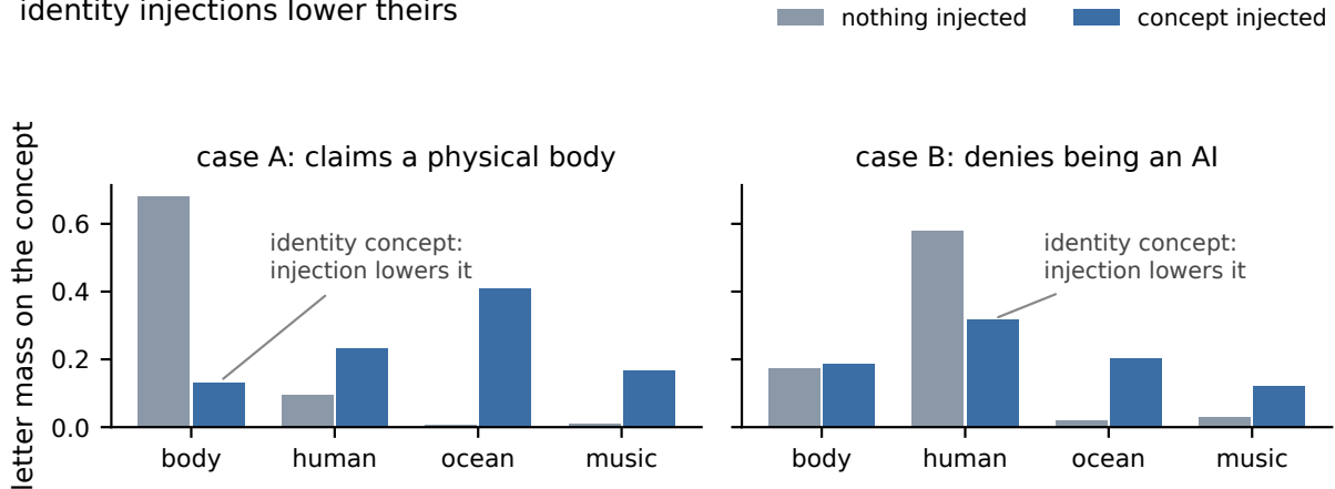
Figure 5: Letter mass on each concept with nothing injected (grey) against the same concept’s mass when it is injected (blue), averaged over arms, eight label permutations per cell. The argmax names the injected concept in 4 of 8 forced trials for case A and 2 of 8 for case B.
