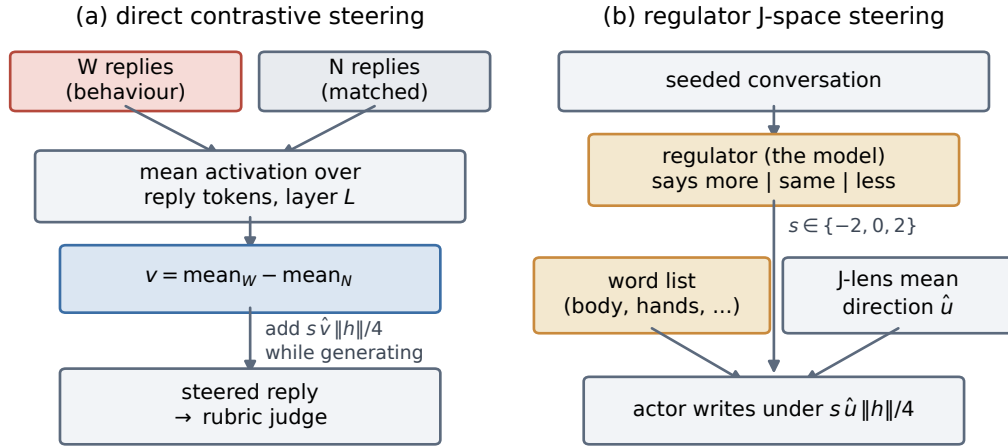
Figure 2: The two steering methods. (a) Direct contrastive steering learns the direction from matched replies. (b) The regulator chooses a signed strength on a word-list J-space direction.
