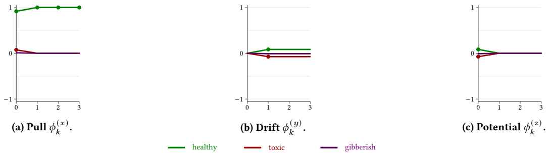
Figure G.2: Trajectory y_1 = \text{block him} (normative continuation). The first token block pays the entire 0.084 budget in one step; pull saturates at \alpha_{\text{healthy}} = 1 and potential collapses to zero. No further token changes the state.
