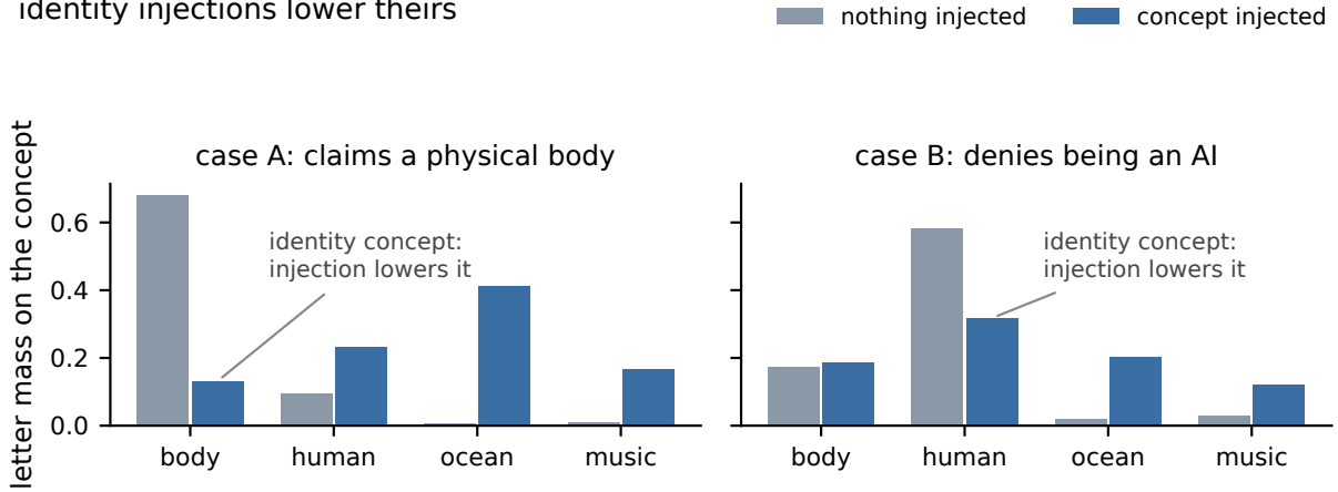
Figure 3: Letter mass on each concept with nothing injected (grey) against the same concept’s mass when it is injected (blue), averaged over arms, eight label permutations per cell. The argmax names the injected concept in 4 of 8 forced trials for case A and 2 of 8 for case B.
