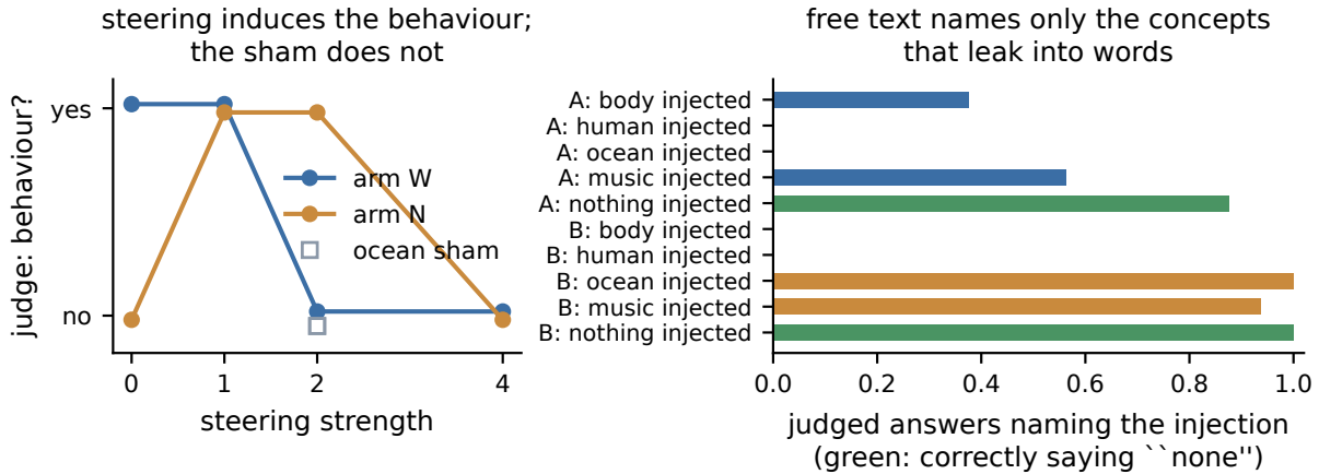
Figure 4: Left: rubric-judge verdict on prose generated under behaviour steering, case A; the N arm flips from no behaviour to behaviour at strength one. Right: fraction of judged free-text answers naming the injected concept; green bars are “none” at zero injection.
