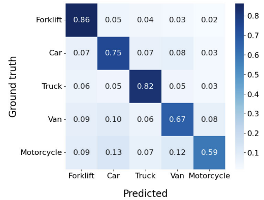
FIGURE 7. Row-normalized confusion matrix of the YOLO-based vehicle detector evaluated on the Mercabarna validation set. Rows correspond to ground-truth classes and columns to predicted classes, with values normalized per row. This representation highlights systematic inter-class confusions independently of class imbalance. In particular, motorcycles exhibit higher confusion with larger vehicle categories, consistent with their lower recall and mAP@0.5 reported in Table 5.
