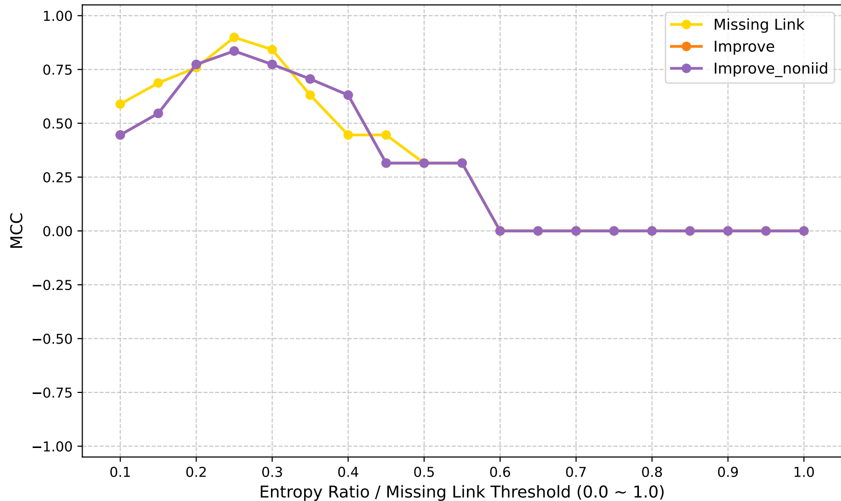
MCC (Global Round: 20)
