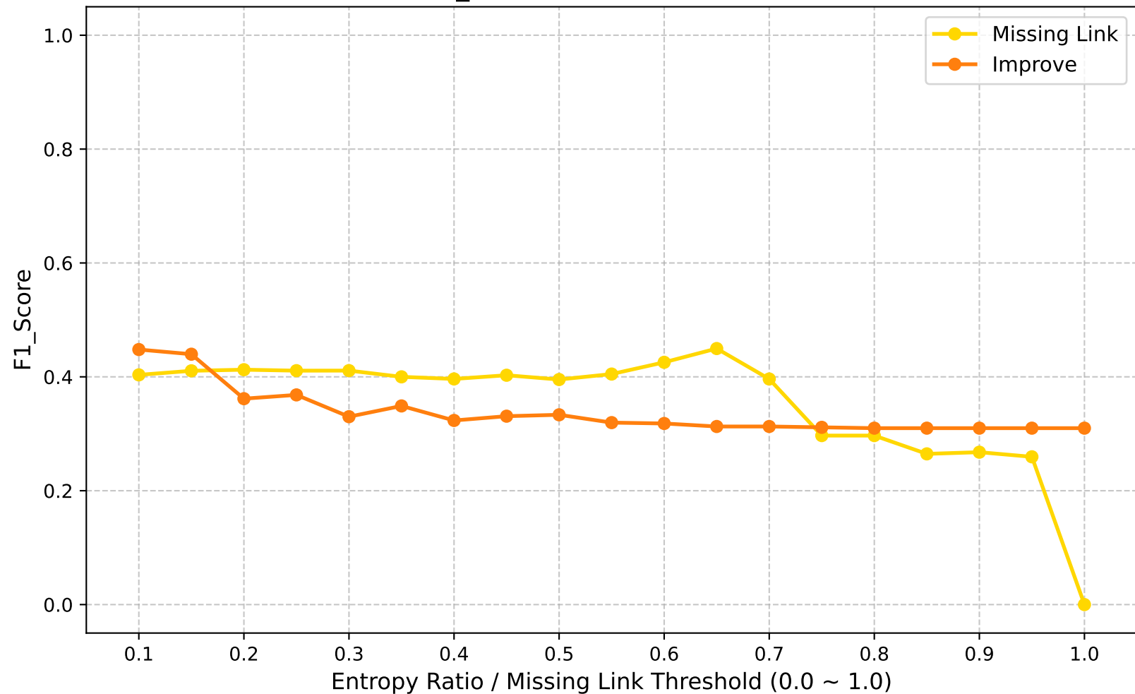
F1_Score (Global Round: 30)
