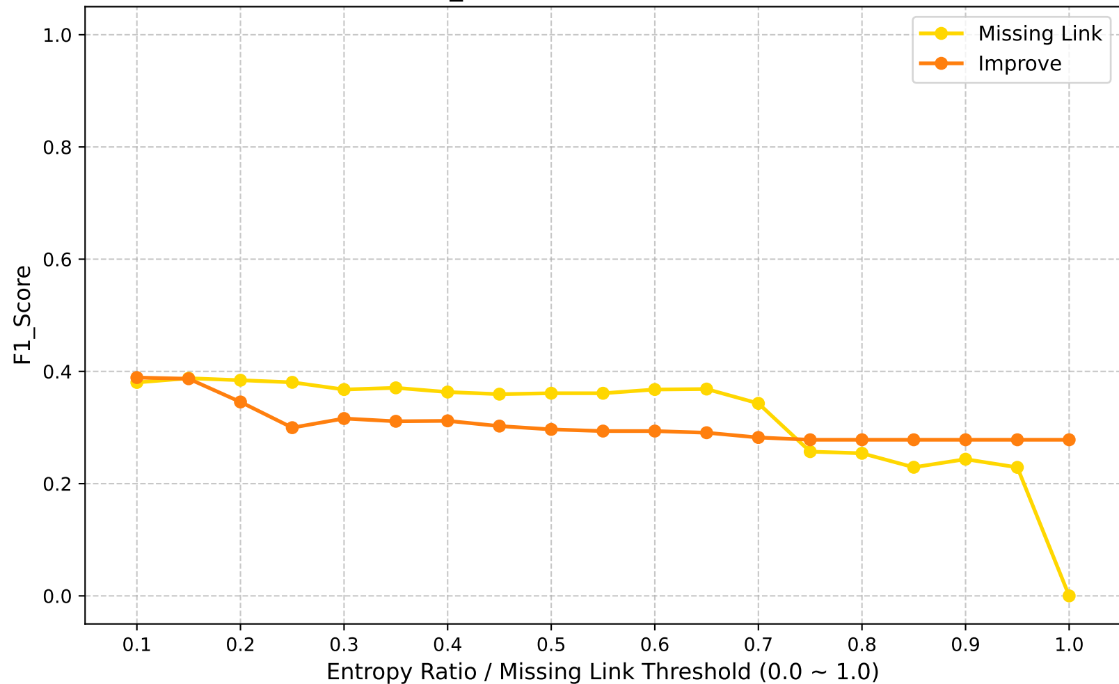
F1_Score (Global Round: 70)
