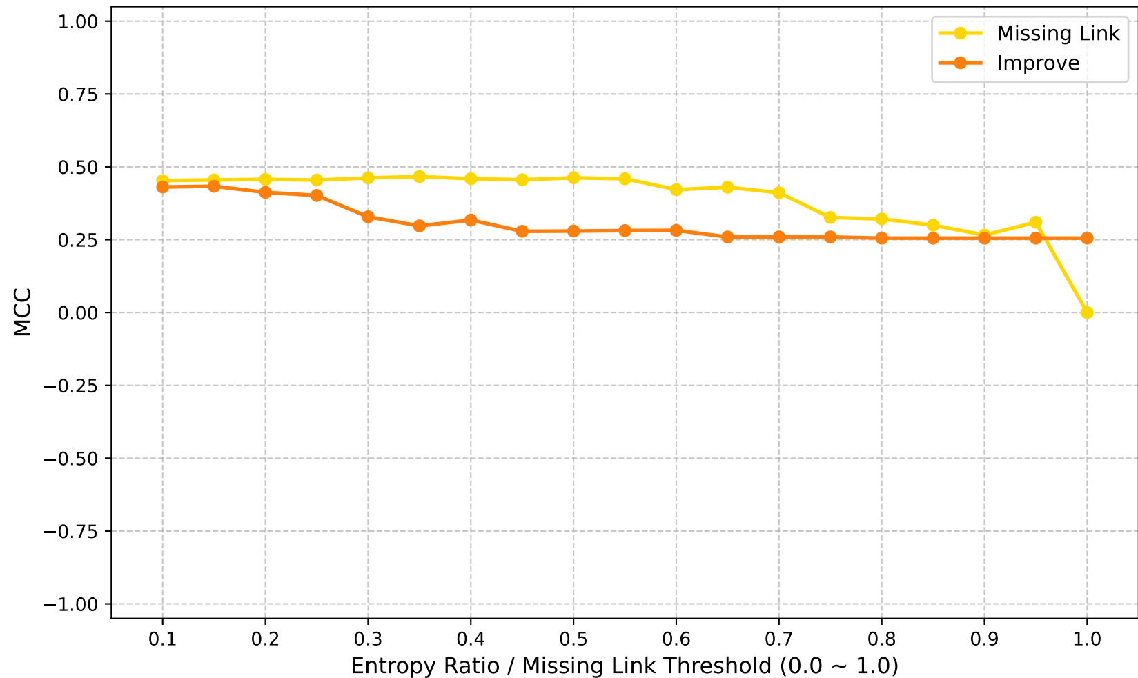
MCC (Global Round: 45)
