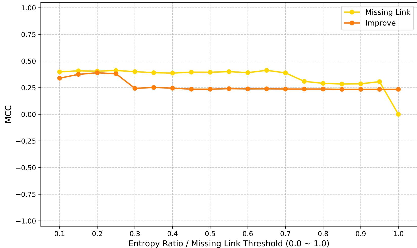
MCC (Global Round: 75)
