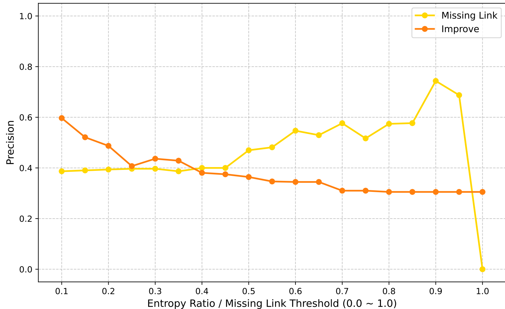
Precision (Global Round: 100)
