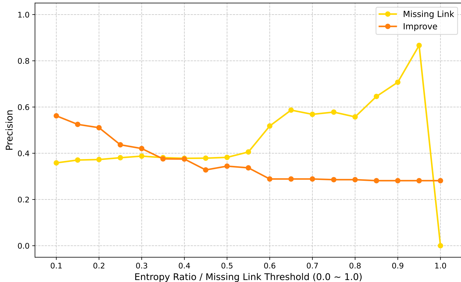
Precision (Global Round: 35)
