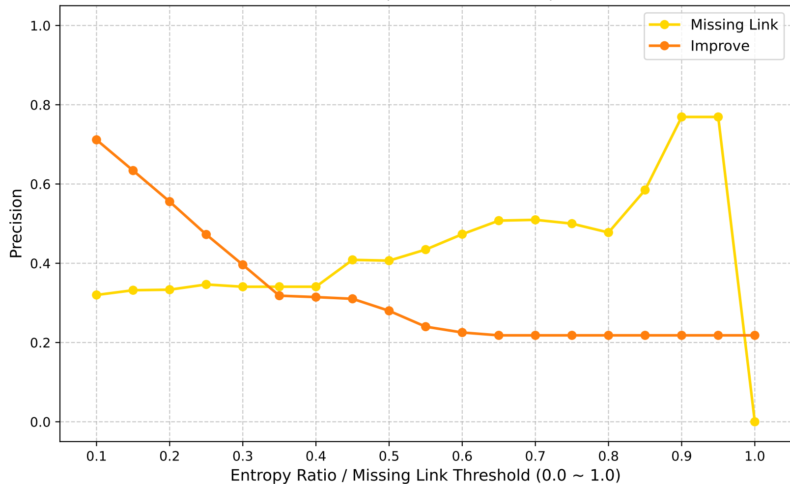
Precision (Global Round: 40)
