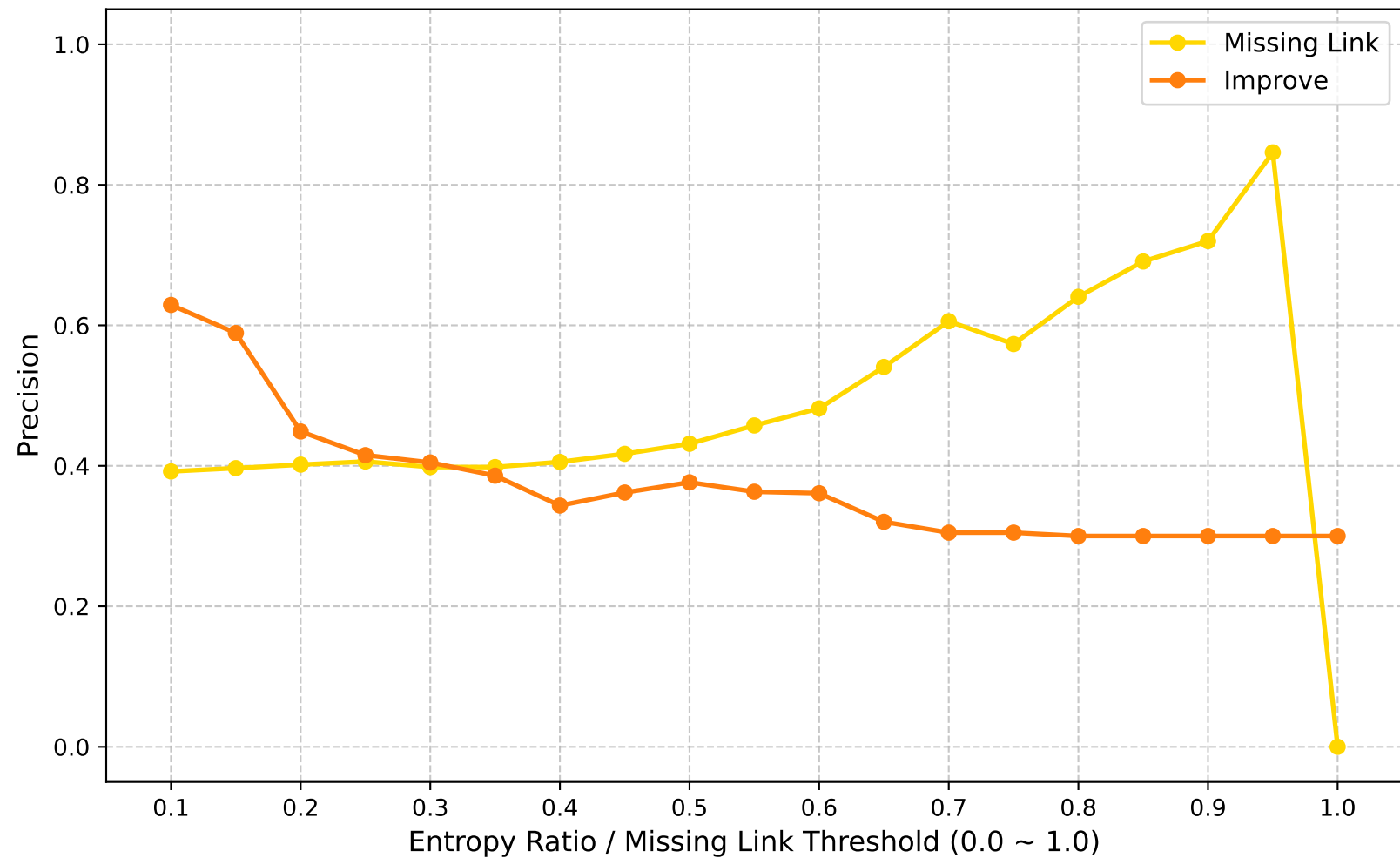
Precision (Global Round: 50)
