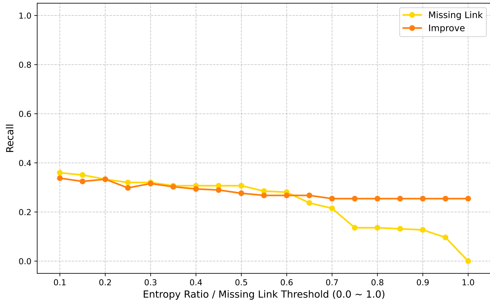
Recall (Global Round: 100)
