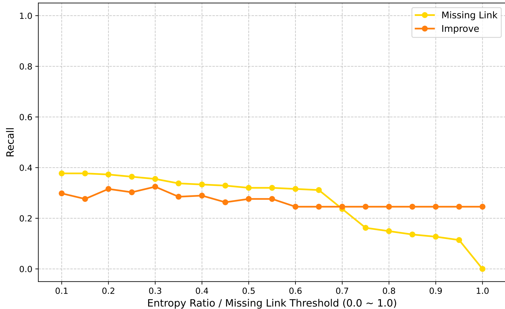
Recall (Global Round: 35)
