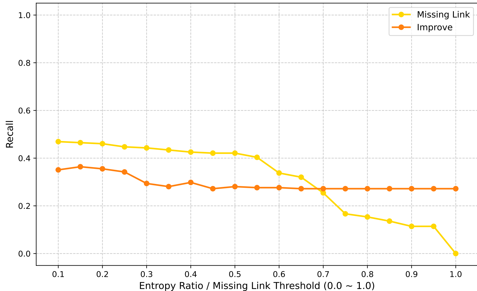
Recall (Global Round: 45)
