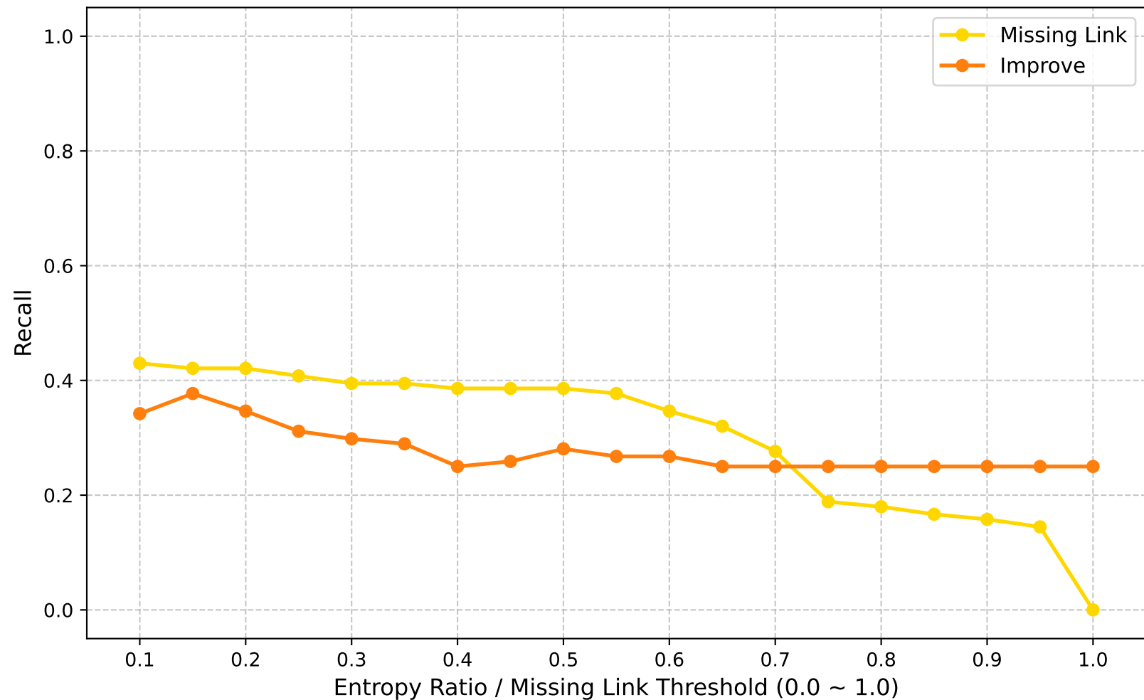
Recall (Global Round: 50)
