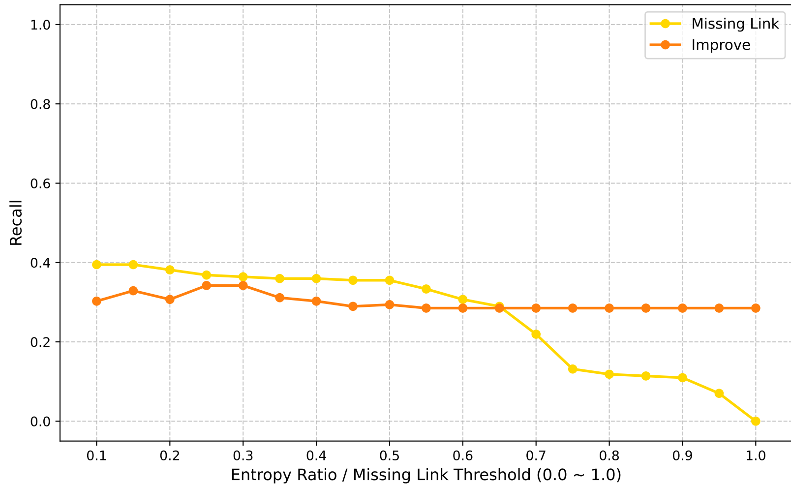
Recall (Global Round: 55)
