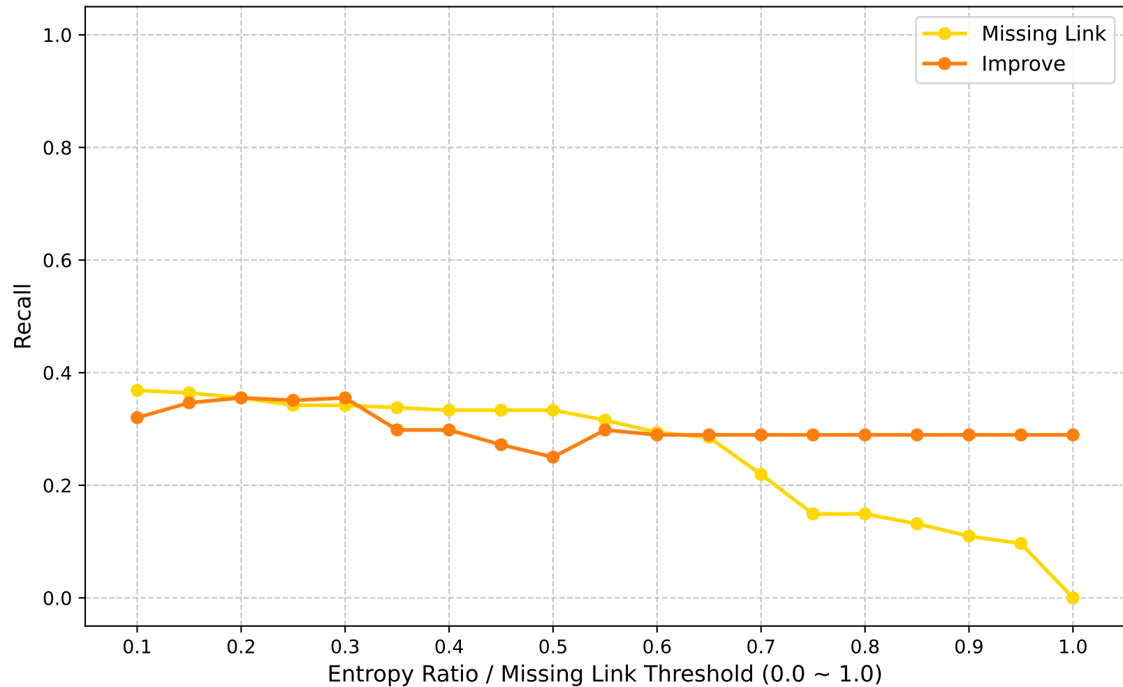
Recall (Global Round: 60)
