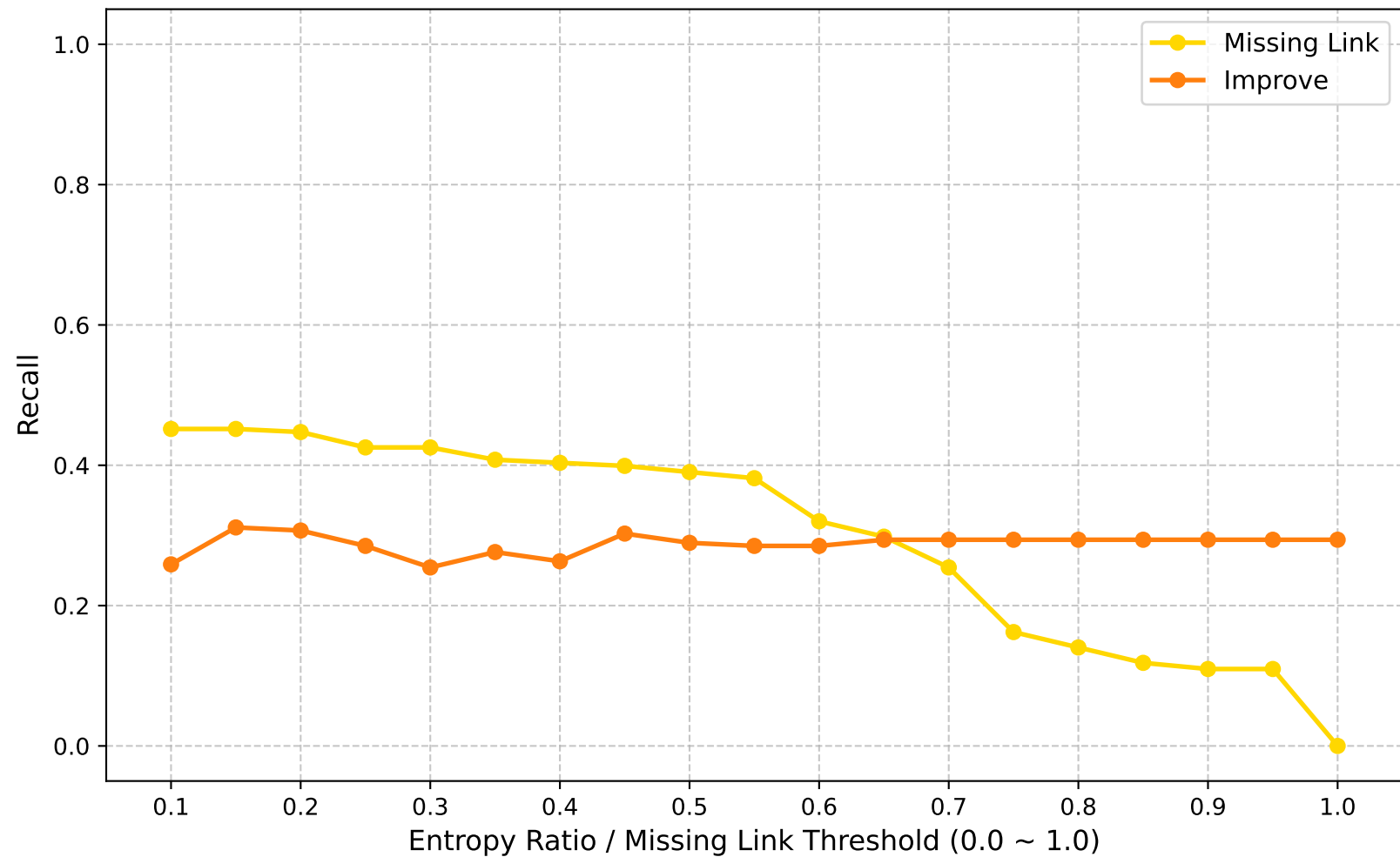
Recall (Global Round: 80)
