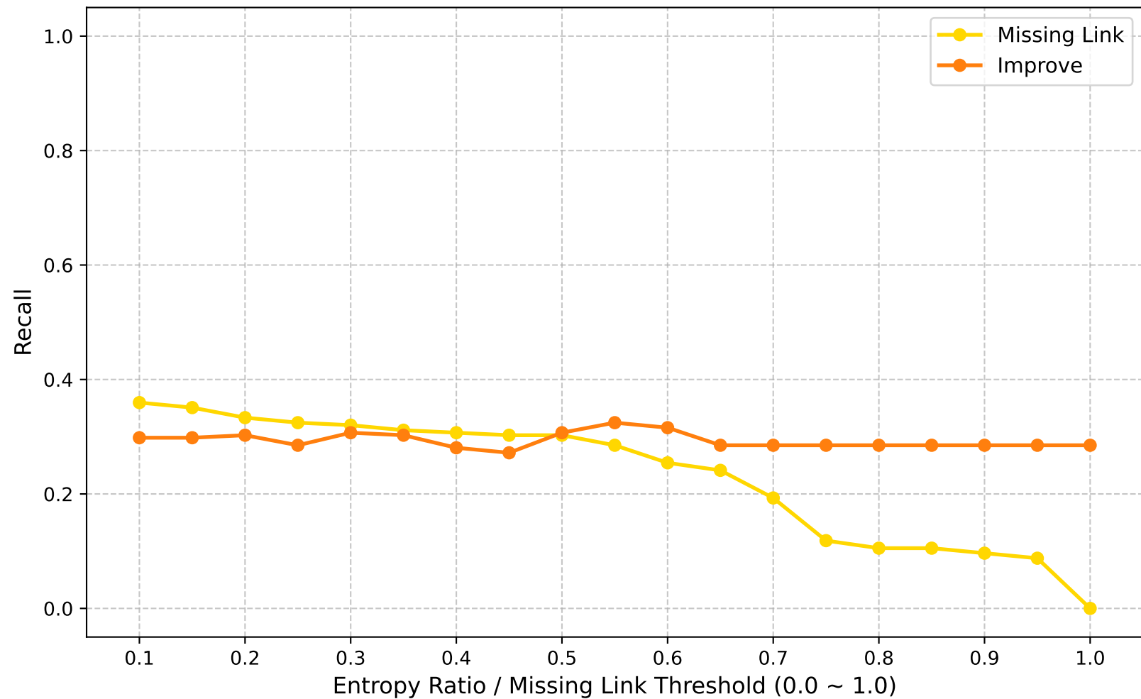
Recall (Global Round: 95)
