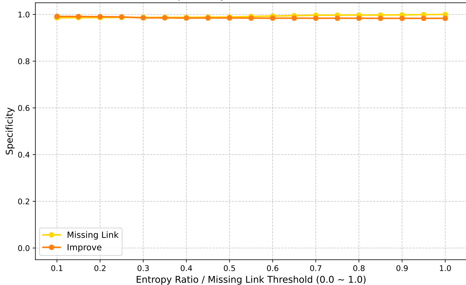
Specificity (Global Round: 75)
