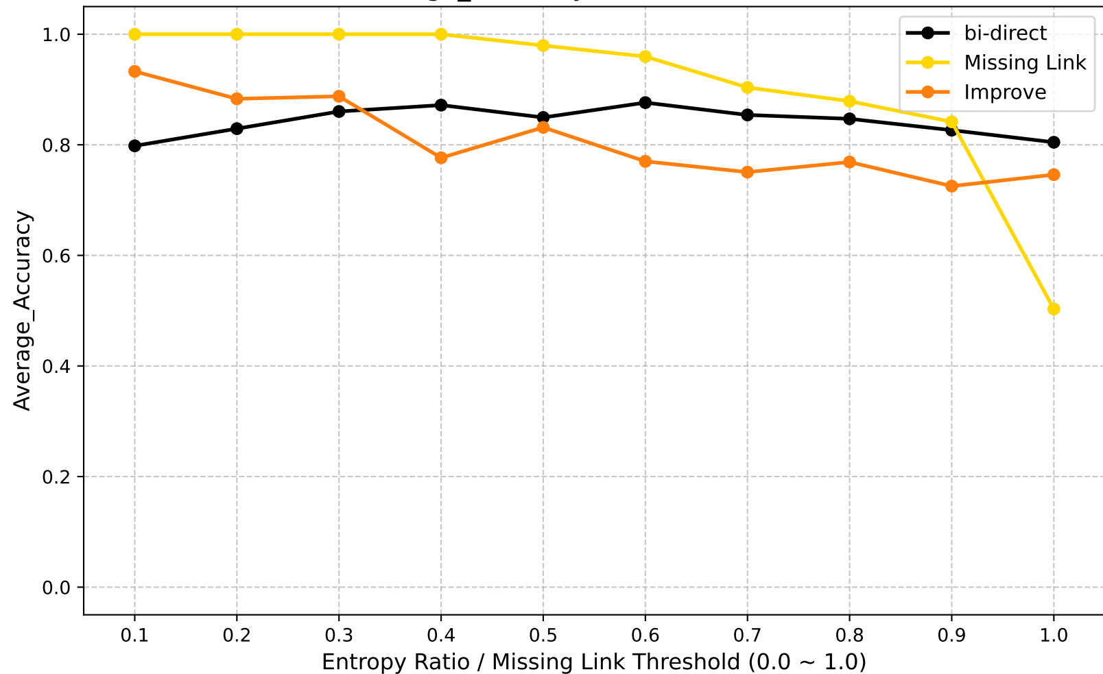
Average_Accuracy (Global Round: 25)
